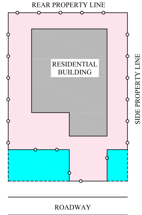
METER LOCATION - SERVICE PEDESTAL
