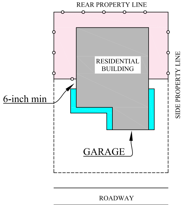
METER LOCATION - BUILDING MOUNTED
